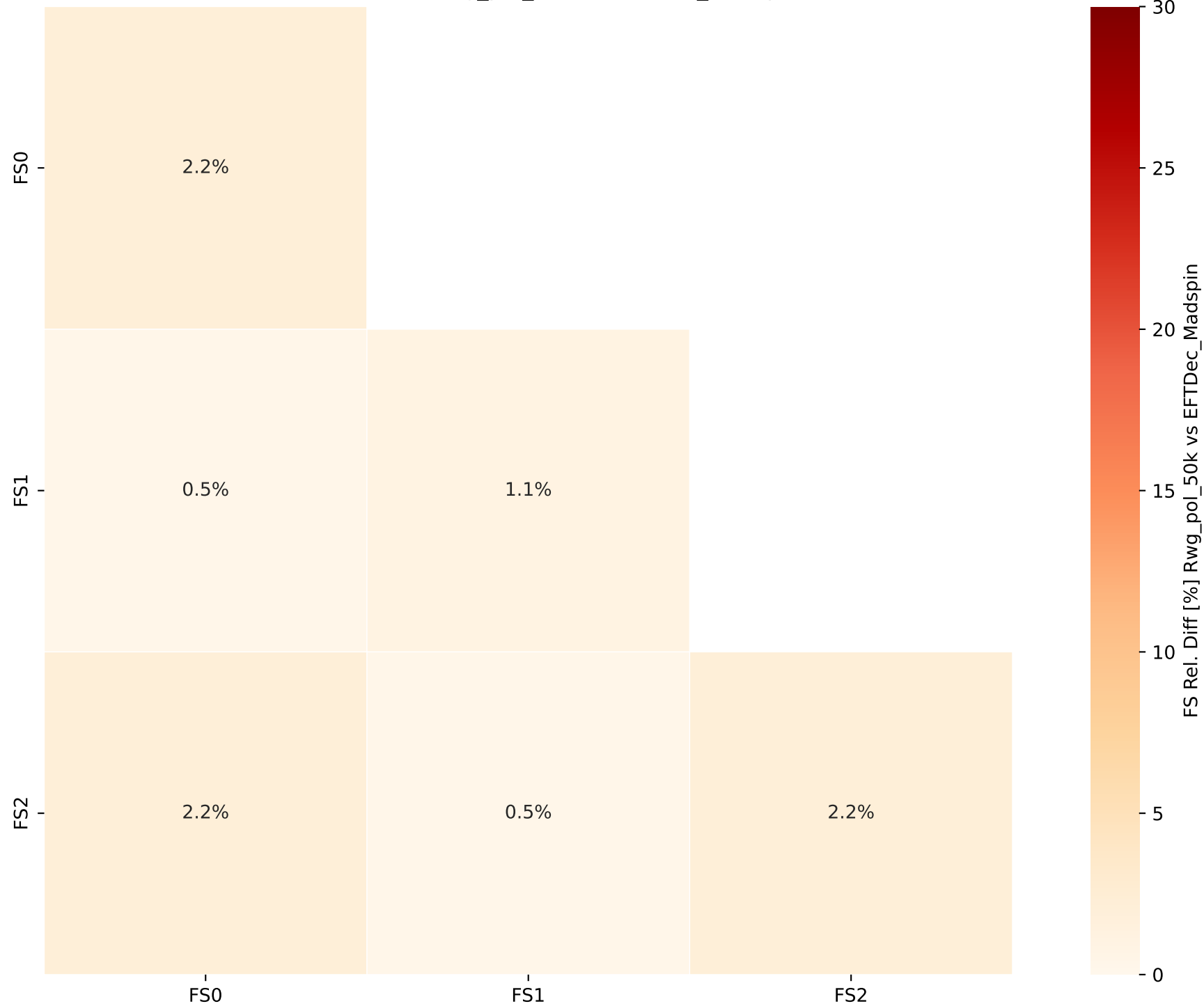
FS Rel. Diff [%] Rwg_pol_50k vs EFTDec_Madspin
